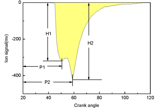
Figure. 6. Parametrization of the ionization signal.
